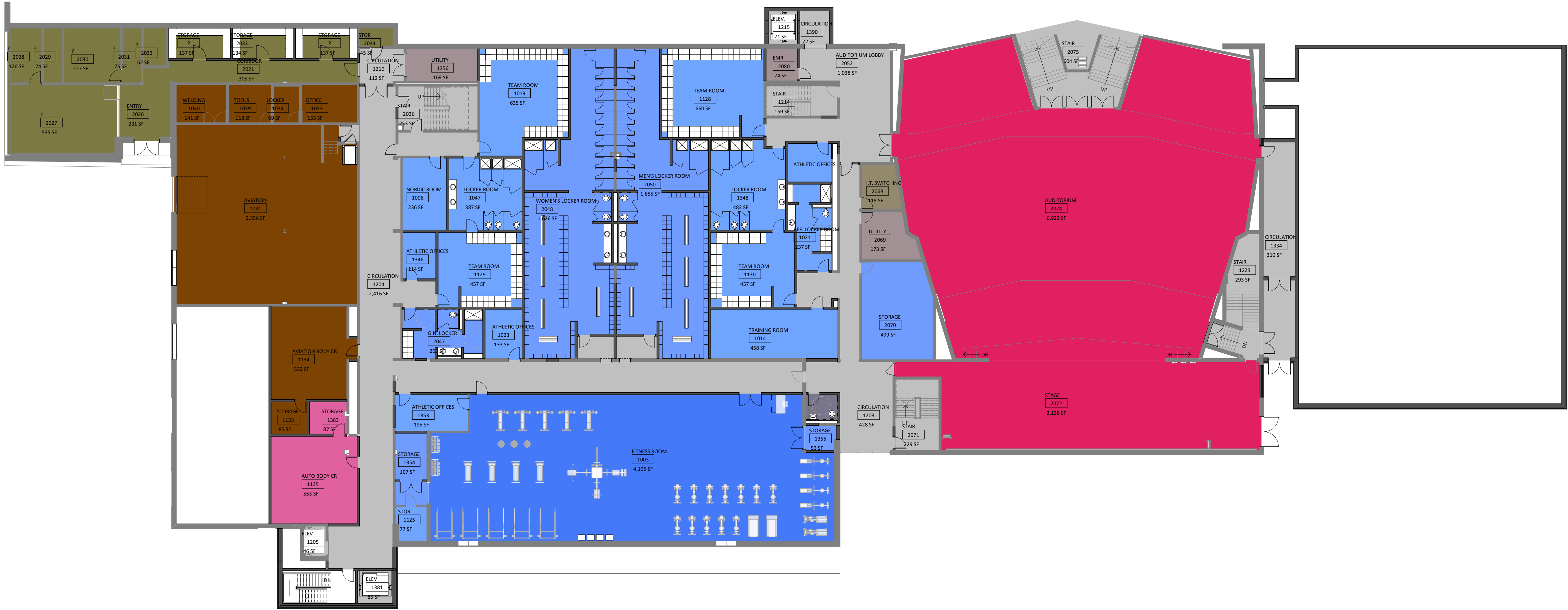
2 PROPOSED BUILDING A/B - LEVEL 2 SCALE: 1/16" = 1'-0"
